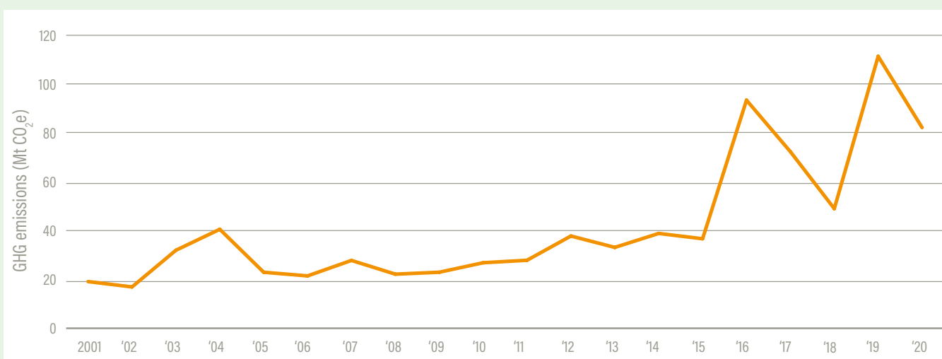
Figure 7: Estimated annual gross forest greenhouse gas emissions across natural and mixed UNESCO World Heritage sites
