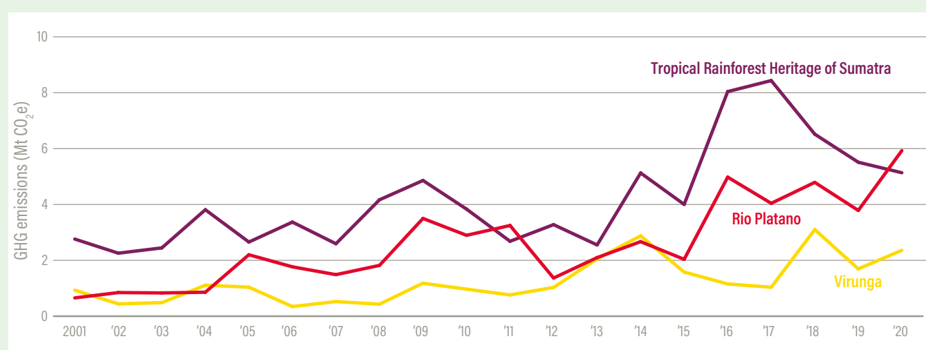
Figure 12: Estimated annual gross forest greenhouse gas emissions at select natural UNESCO World Heritage sites subject to land-use pressures
