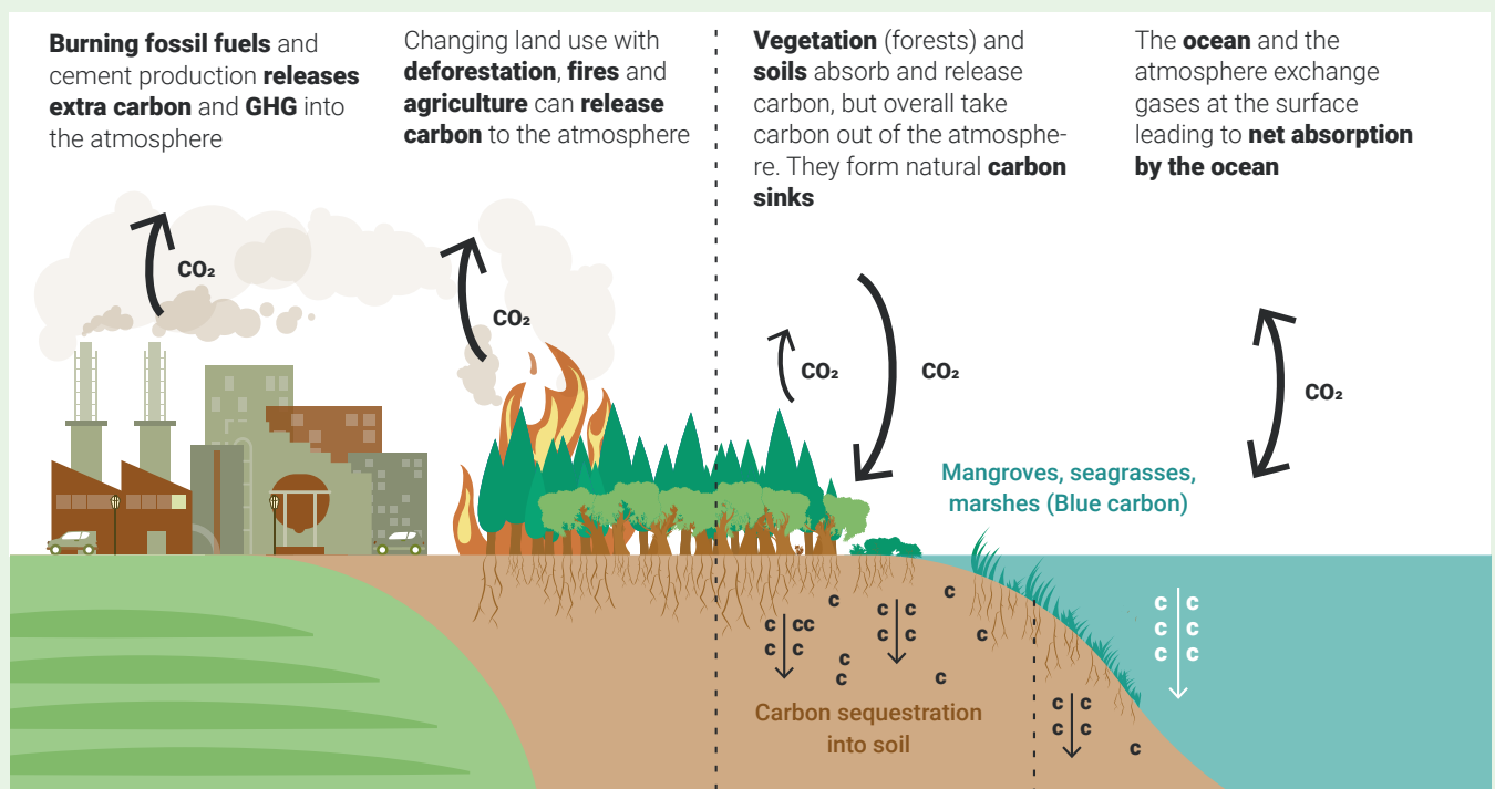
Figure 2: Simplified overview of the movement of carbon through the planet's living (biotic) components, sometimes referred to as the "fast" portion of the global carbon cycle.
