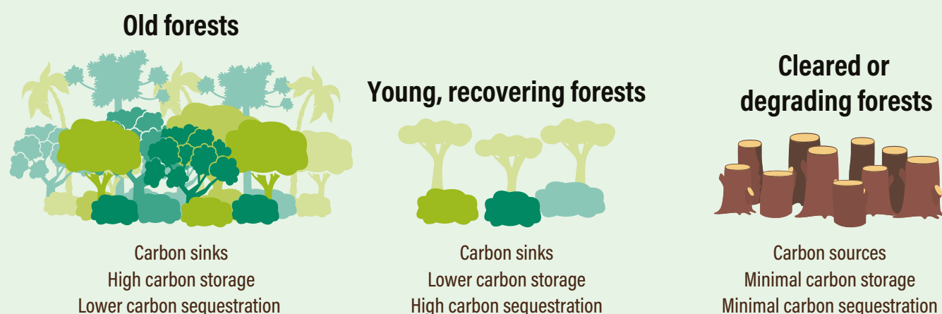
Figure 3: Carbon storage, emissions, and removals across different forest and land use profiles.
