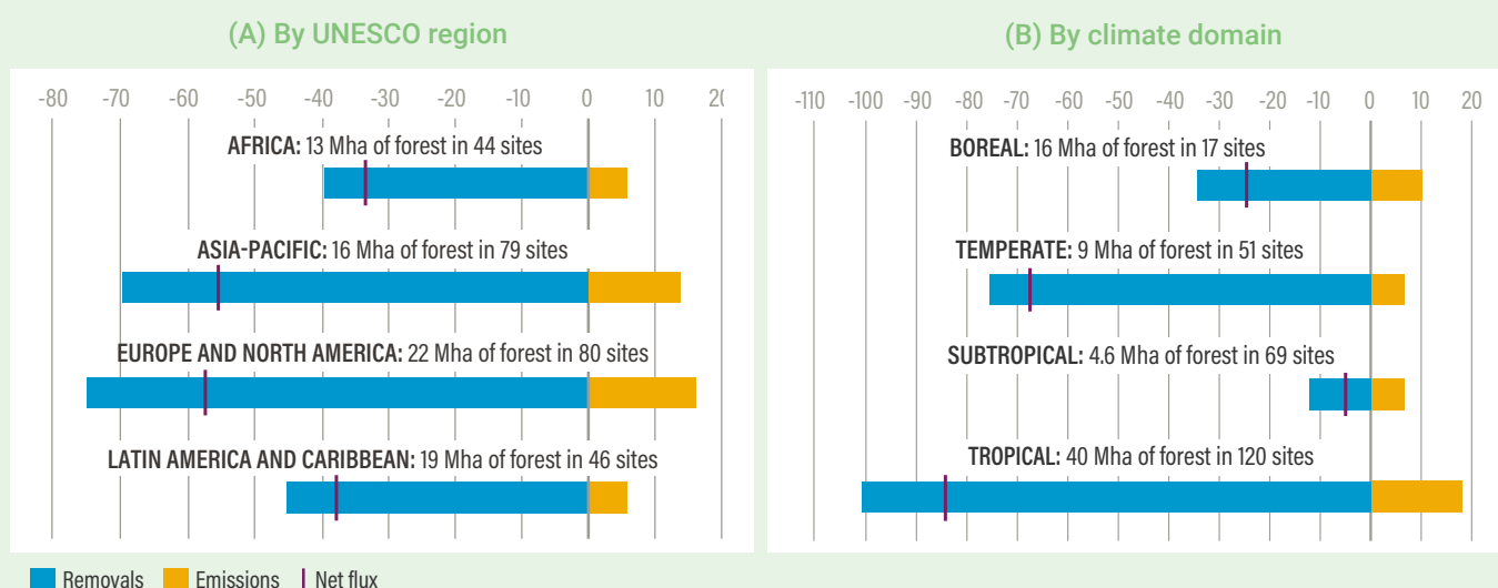
Figure 4: Forest greenhouse gas fluxes (average 2001-2020, Mt CO 2 e/yr) in natural and mixed UNESCO World Heritage sites aggregated by (A) UNESCO region; and (B) climate domain.
