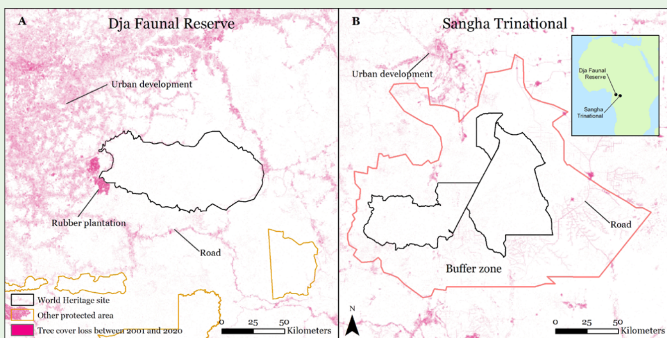
Figure 13: Buffer zone management can reduce pressures on sites. Tree cover loss around (A) Dja Faunal Reserve (Cameroon), which does not have a buffer zone, has been significantly higher than in (B) Sangha Trinational (Cameroon, Central African Republic, Republic of the Congo), which does have a buffer zone.
