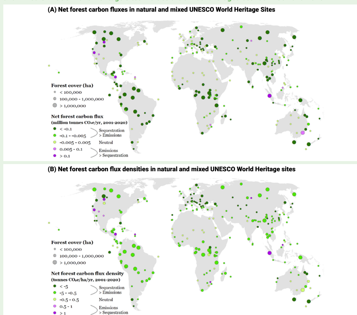
Figure 5: (A) Net forest carbon fluxes and (B) flux densities (net carbon flux per hectare of forest) in natural and mixed UNESCO World Heritage sites. Values are annual averages between 2001 and 2020.
