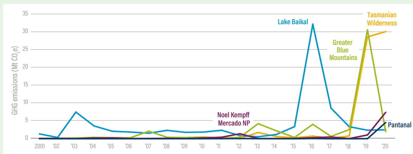
Figure 8: Estimated annual gross forest greenhouse gas emissions among select natural and mixed UNESCO World Heritage sites with substantial fire activity
