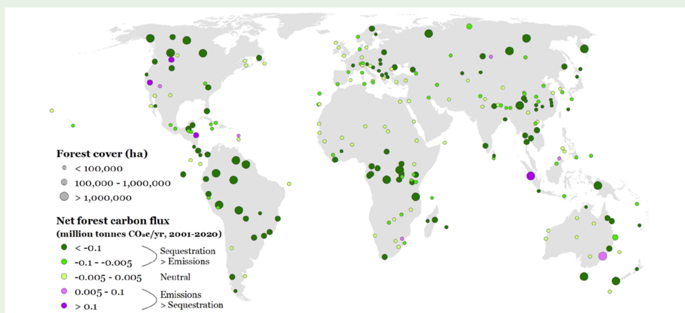
Figure ES 1: Net forest carbon fluxes in natural and mixed UNESCO World Heritage sites. Values are annual averages between 2001 and 2020.
