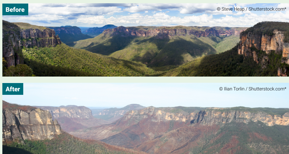
Figure 10: Wide aerial views over the Grose Valley in the Greater Blue Mountains Area World Heritage site in Australia before (top) and after (bottom) massive wildfires. Brown areas indicate burn scars.
