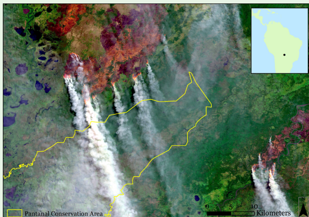
Figure 9: Satellite image showing wildfires close to the Pantanal Conservation Area World Heritage site in Brazil on 14 August 2020. By early October 2020, the wildfires had encroached on a small portion of the site.
